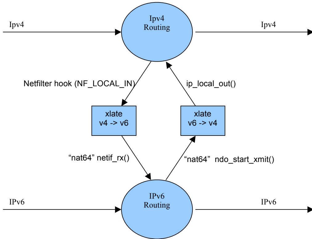
Figure 3: Linux implementation.
