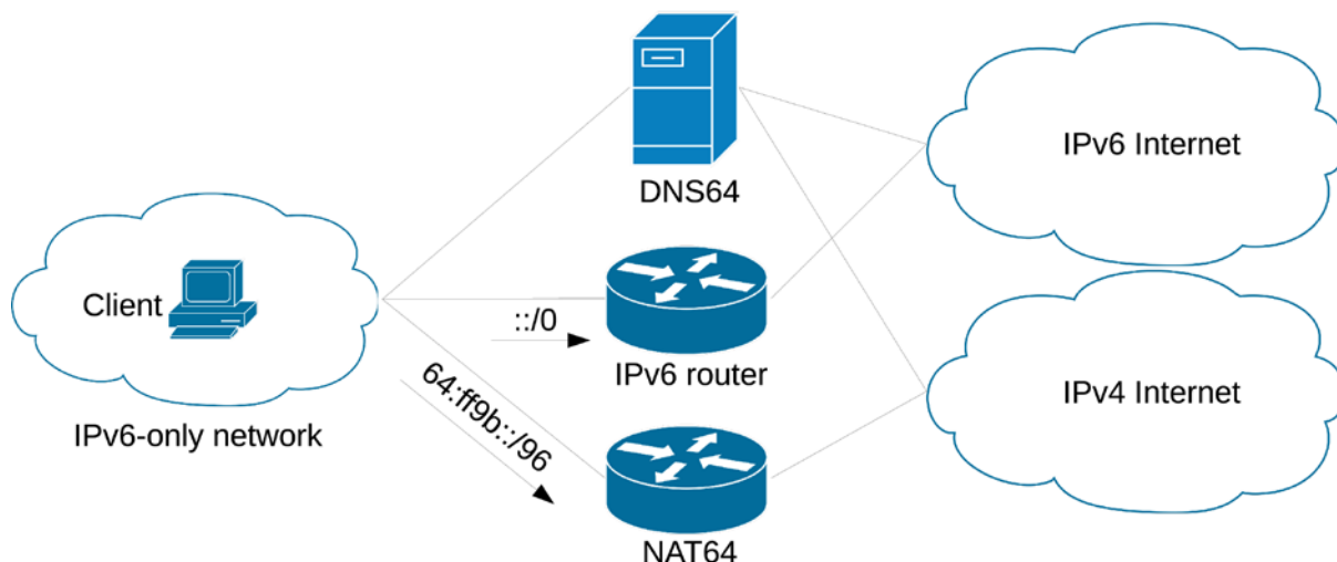
Figure 1: Expected use case. The default NAT64 prefix, 64:ff9b::/96, is routed to the NAT64 device. All other IPv6 traffic is routed to the default IPv6 gateway. The DNS64, which is provisioned to the clients as their default DNS resolver, has both IPv6 and IPv4 connectivity, which it uses for reaching authoritative DNS servers. Note that IPv6 router, DNS64, and NAT64 are logical functions and could conceivably be co-located on the same physical machine.
