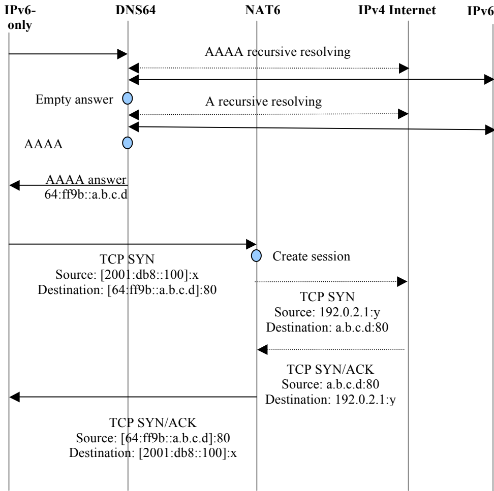
Figure 2: Example connection establishment flow. In this case, the IPv6-only client is attempting a TCP connection to example.com on port 80. There is no AAAA record associated with example.com , and so the DNS64 synthesizes one from the A record, which points to the IPv4 address a.b.c.d , by prefixing it with the NAT64 prefix, which in this case is the default 64:ff9b::/96 . The client then sends a TCP SYN to 64:ff9b::a.b.c.d , port 80. The packet gets routed to the NAT64 device which creates a new session and allocates a binding. It changes the source address of the binding created, and converts the IPv6 destination address to IPv4 by removing the prefix. When the SYN/ACK reply is received, the NAT64 does the reverse operation and forwards the IPv6 packet to the client. The rest of the connection operates in the same fashion.
